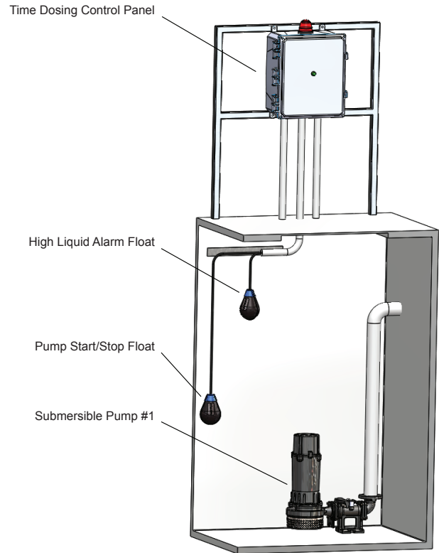
Typical Installation of Simplex Time Dosing Control Panel
